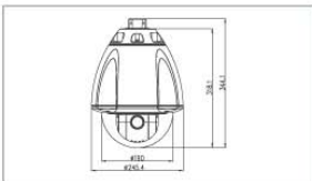
Outdoor Housing (SK-H241)
