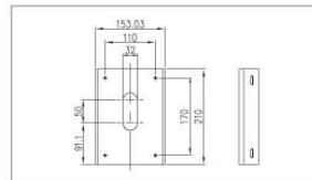
Pole Mount Adaptor (SK-AB18)
