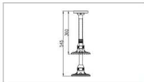
Pendant Mount Bracket (Out door) (SK-AB12)
