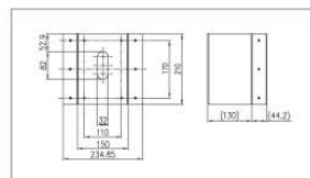
Corner Mount Adaptor (SK-AB09)
